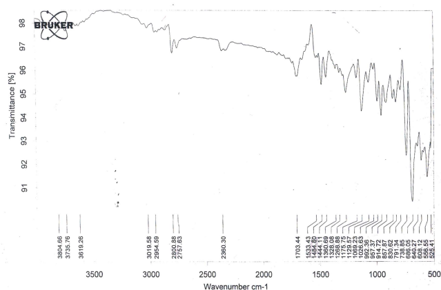
Figure 4.1 FTIR/ATR spectra of Cinnarizine (observed)
